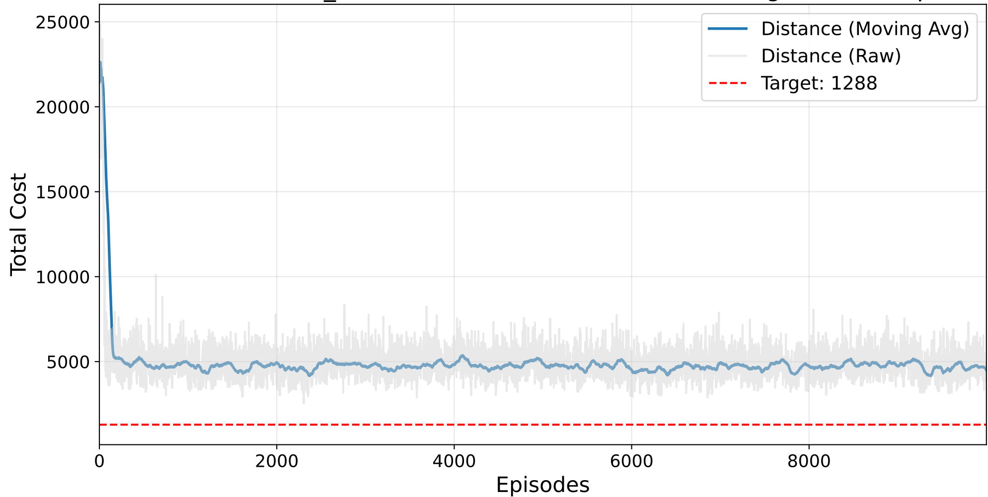
Final RANDOM_SEARCH Masked AutoRL-SOP Training - ESC47.sop
